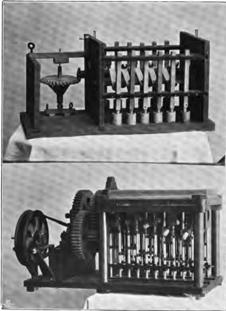
POWDER-MACHINES.
